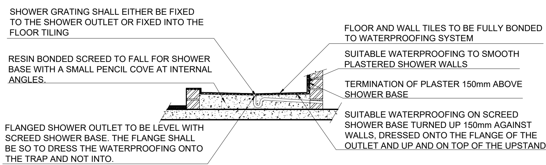
SHOWER BASE DETAIL SCALE 1:50
