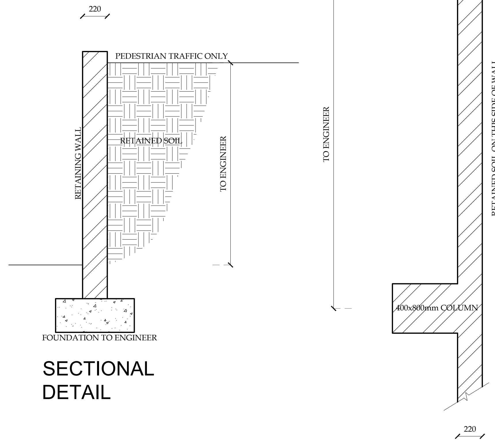
TYPICAL RETAINING WALL DETAIL SCALE 1:20
