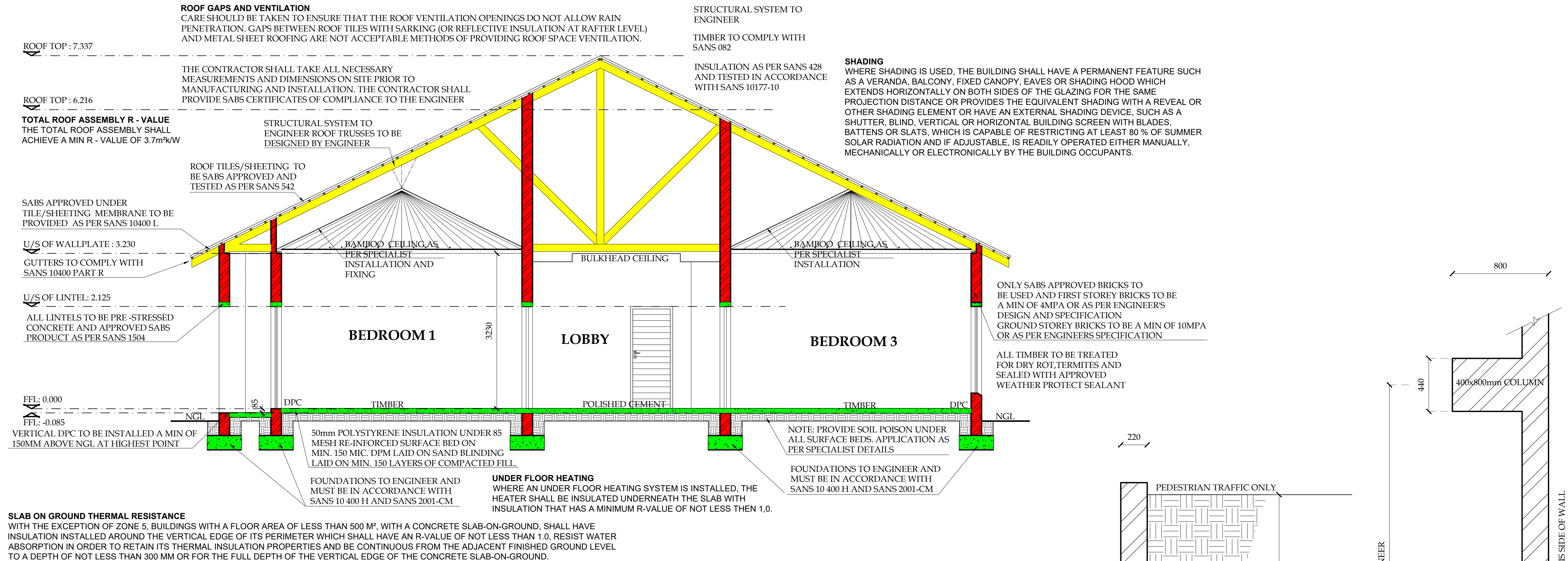
SECTION C-C SCALE 1:50
