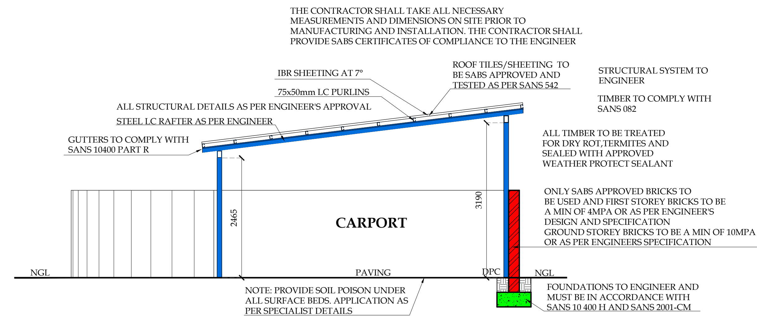
SECTION D-D SCALE 1:50
